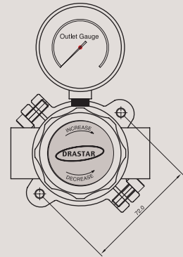
Mounting Bracket Option
